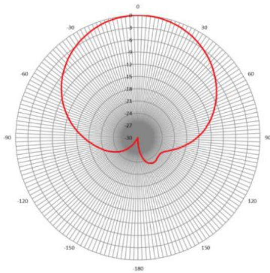
GAIN (normalized to 0dB)
